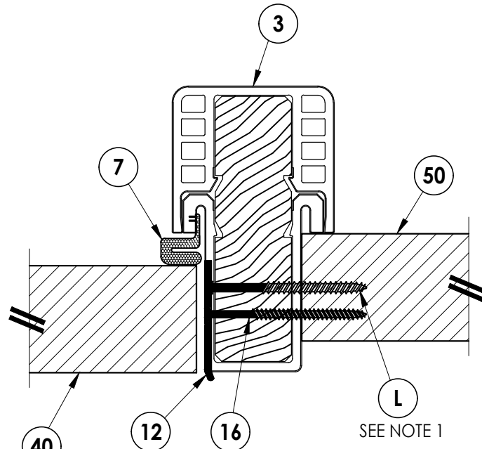
6 4 HORIZONTAL CROSS SECTION Outswing shown (Inswing similar)
