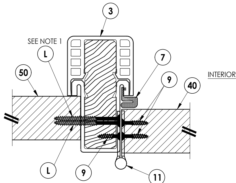
5 4 HORIZONTAL CROSS SECTION Outswing shown (Inswing similar)
